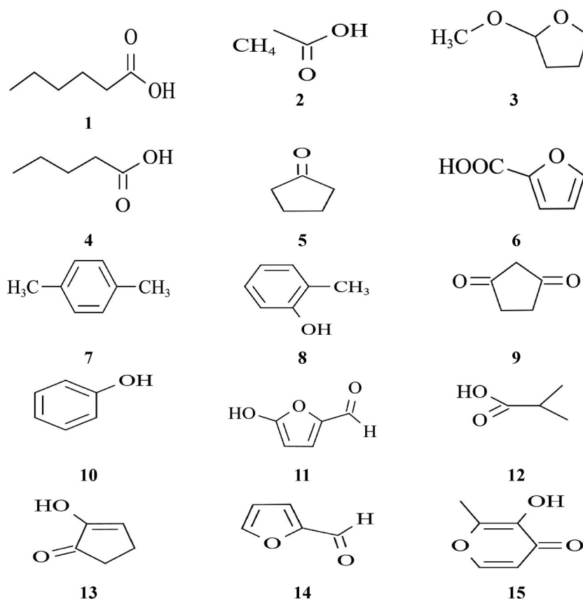
Fig. 2. Structure of chemical composition of wood vinegar. Note: 1. Hexanoic acid, 2. Propionic acid, 3. Methoxytetrahydrofuran, 4. Valeric acid, 5. Cyclopentanone, 6. Furanicarboxylic acid, 7. P-xylene, 8. Methylphenol, 9. Hexyl Dione, 10. PPhenol, 11. Hydroxymethyl-2-furaldehyde, 12. Dimethylpropionieacid, 13. 2-Hydroxy-2-cyclopenten-1-one, 14. Furfural, 15. Maltol.
